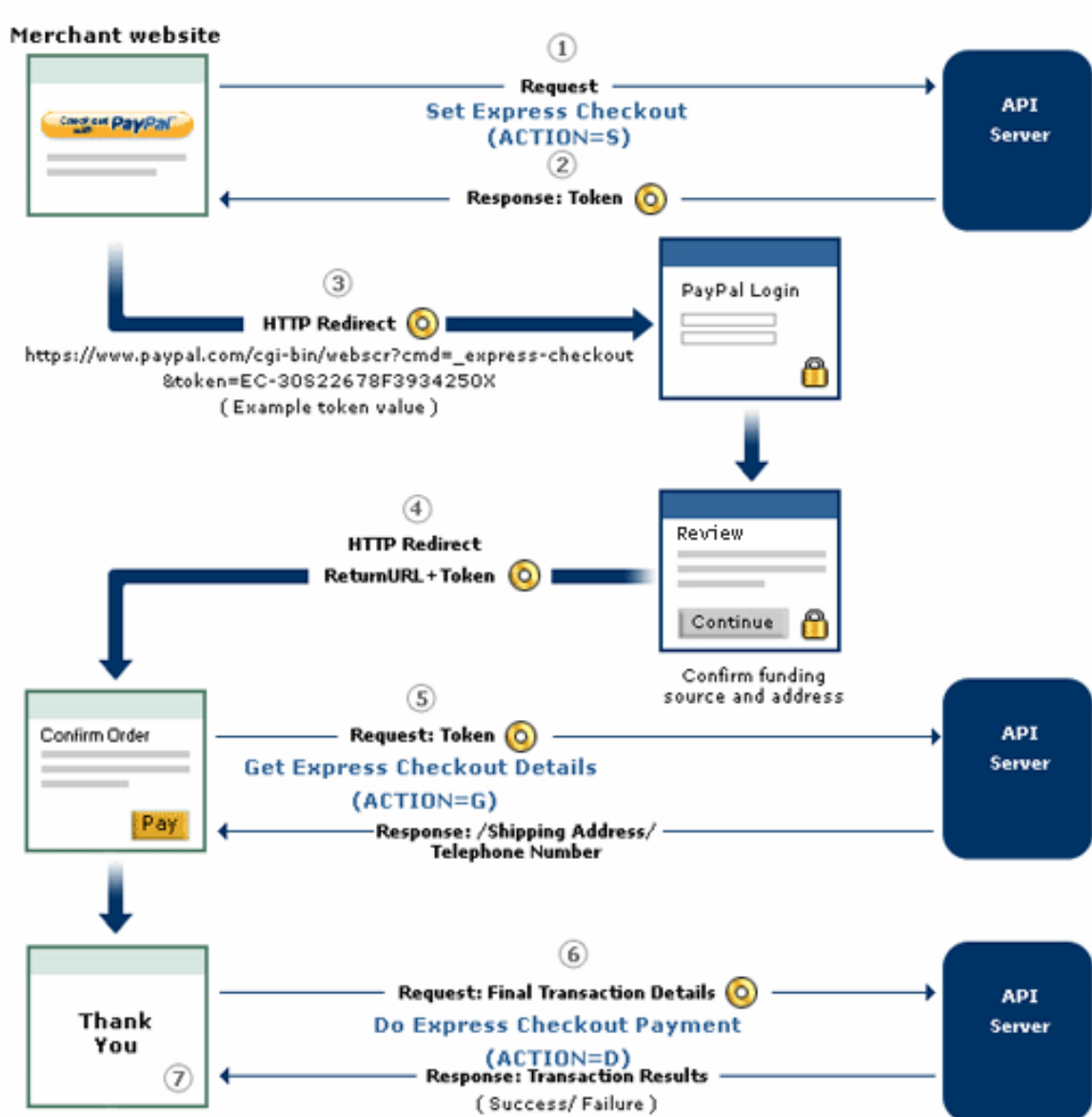
FIGURE 1.1 Express Checkout flow
